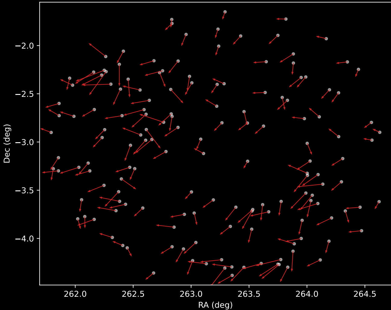
APOGEE DR17 Cluster 6 Proper Motion Vectors (n=153)
