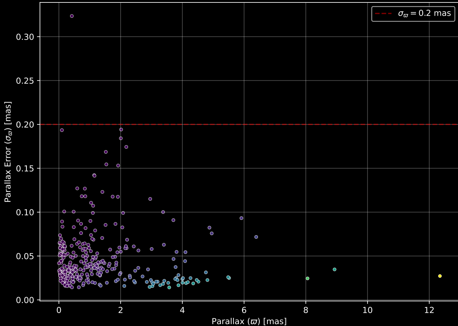
APOGEE DR17 Field: [ORPHAN-1] Parallax Quality (n= 320)
