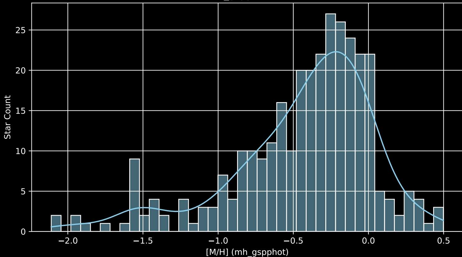
APOGEE DR17 Field: [ORPHAN-1 [M/H] (mh_gspphot) (n= 319)
