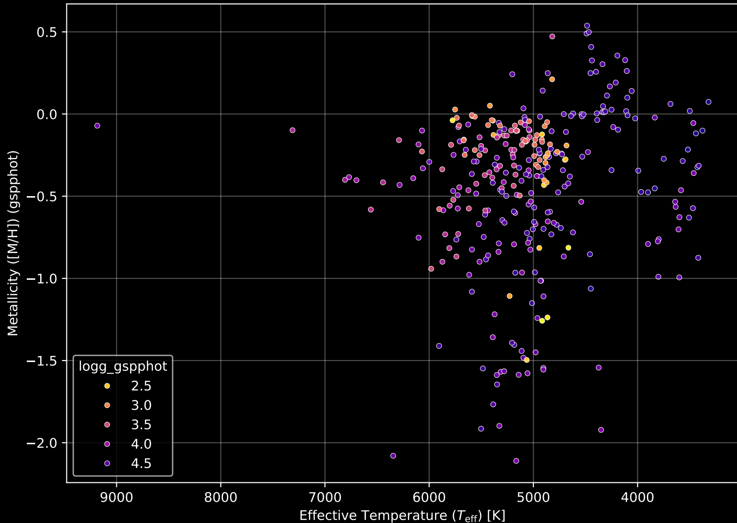
APOGEE DR17 Field: [ORPHAN-1] Stellar Population Parameters (n= 320)
