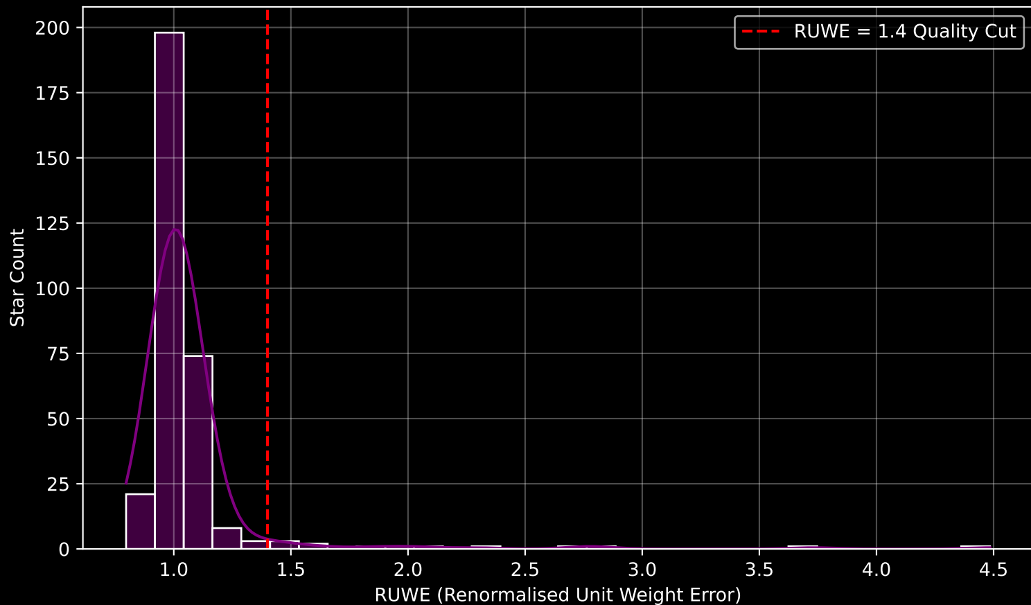
GAPOGEE DR17 Field [ORPHAN-1] RUWE Distribution (n= 317)
