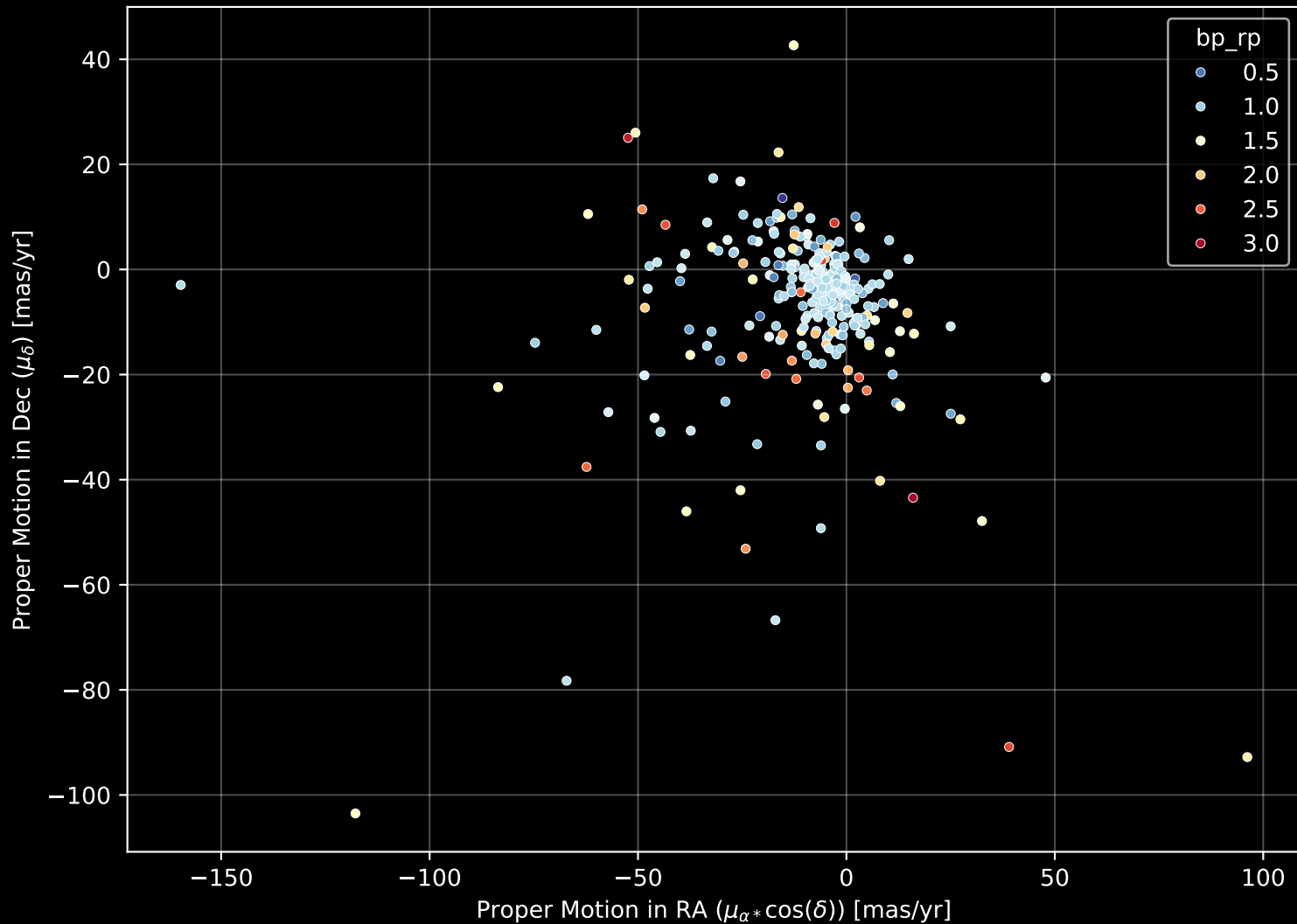
APOGEE DR17 Field: [ORPHAN-1] Proper Motion Diagram (n= 320)
