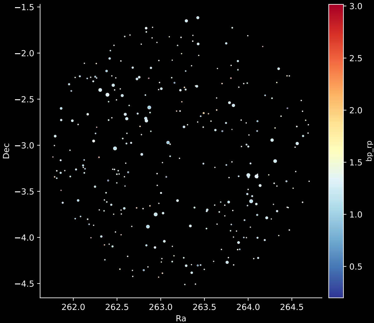
APOGEE DR17 Field: [ORPHAN-1] Stars: 320
