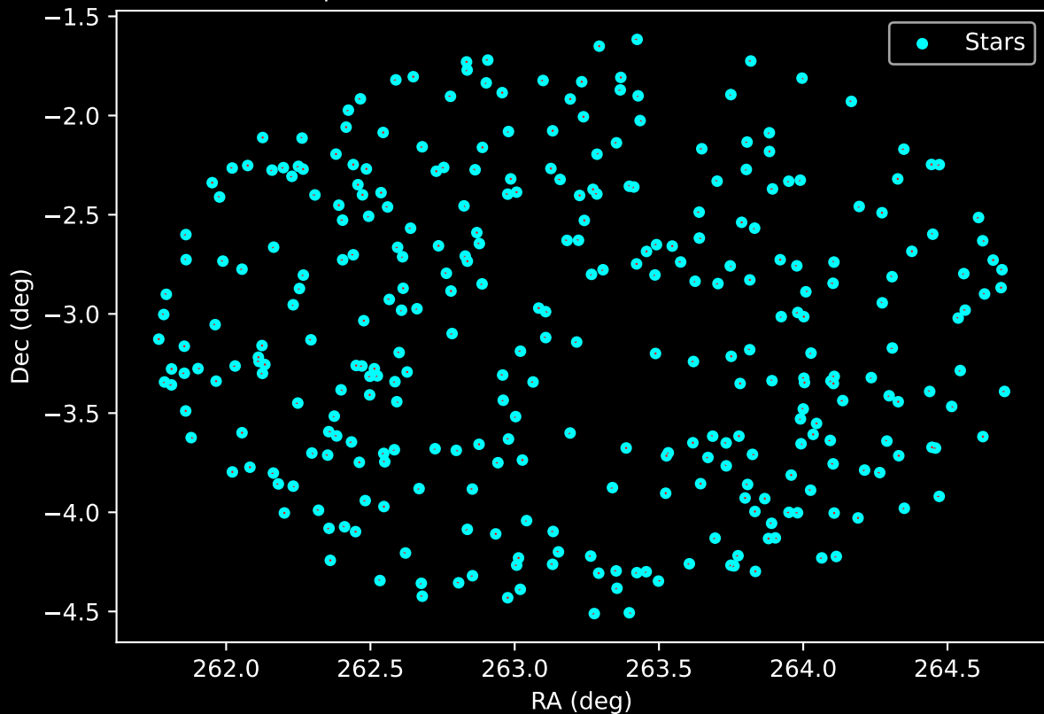
APOGEE DR17 Field: [ORPHAN-1] Proper Motion Vectors for Gaia Star Field (n= 320)
