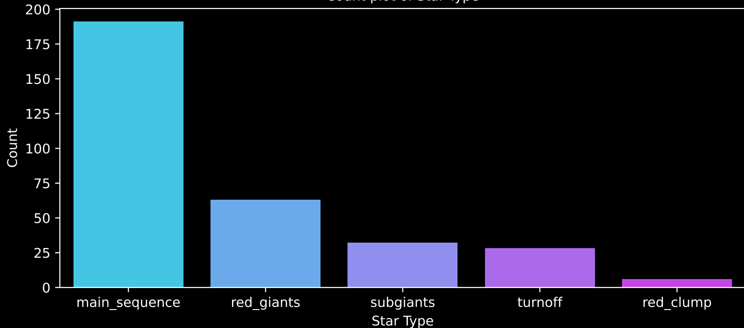
APOGEE DR17 Field: [ORPHAN-1] Count plot of Star Type
